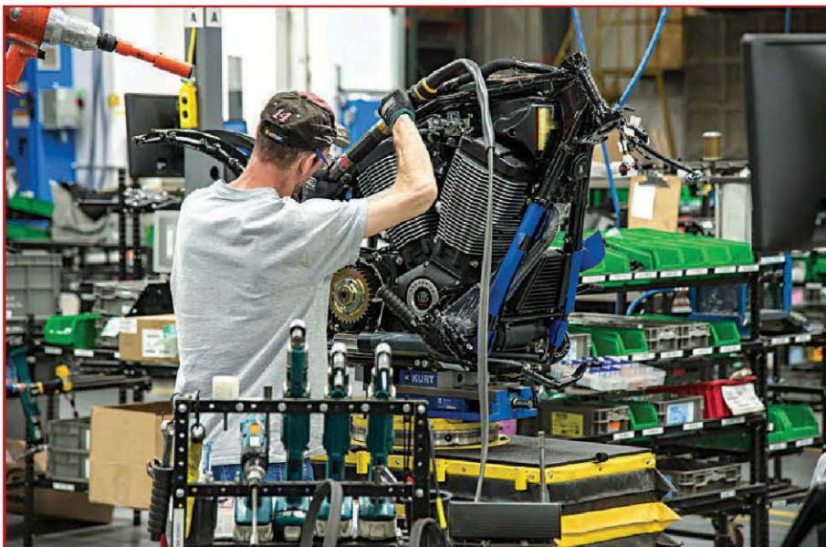
Assembler use DC electric tools for safety-critical and quality-critical fastening applications. Photo courtesy Polaris Industries Inc.
